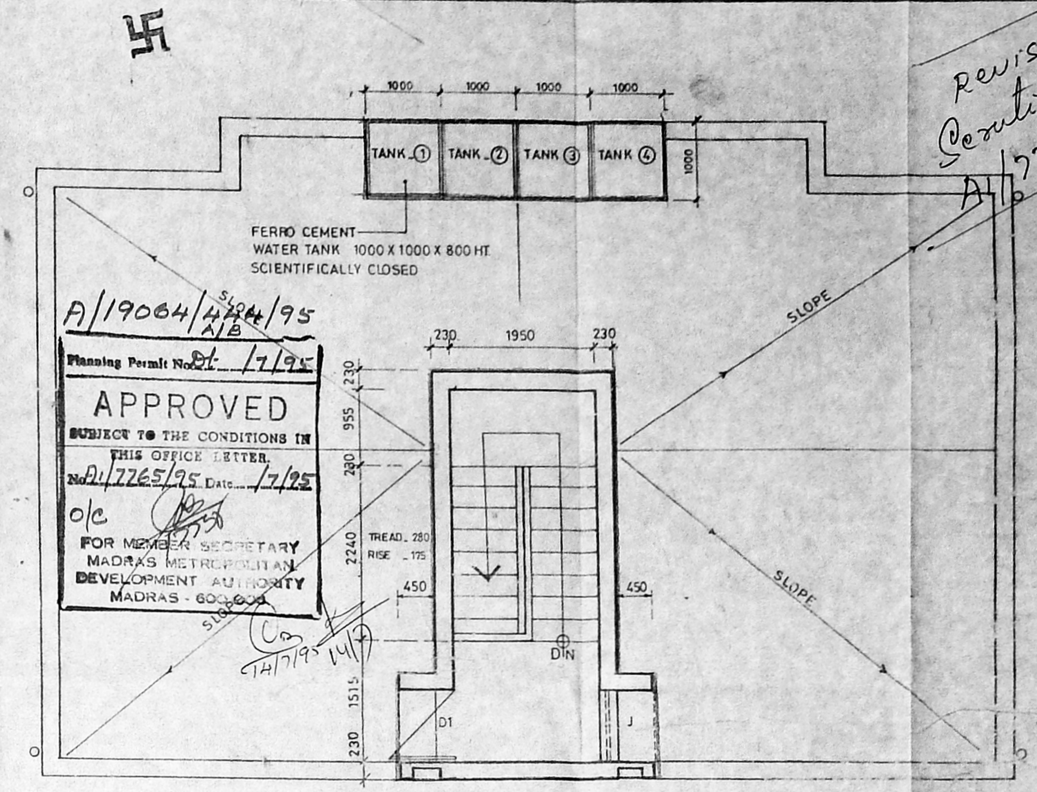
TERRACE PLAN
