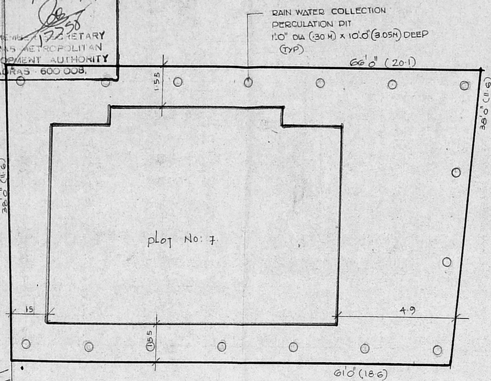
SITE PLAN
