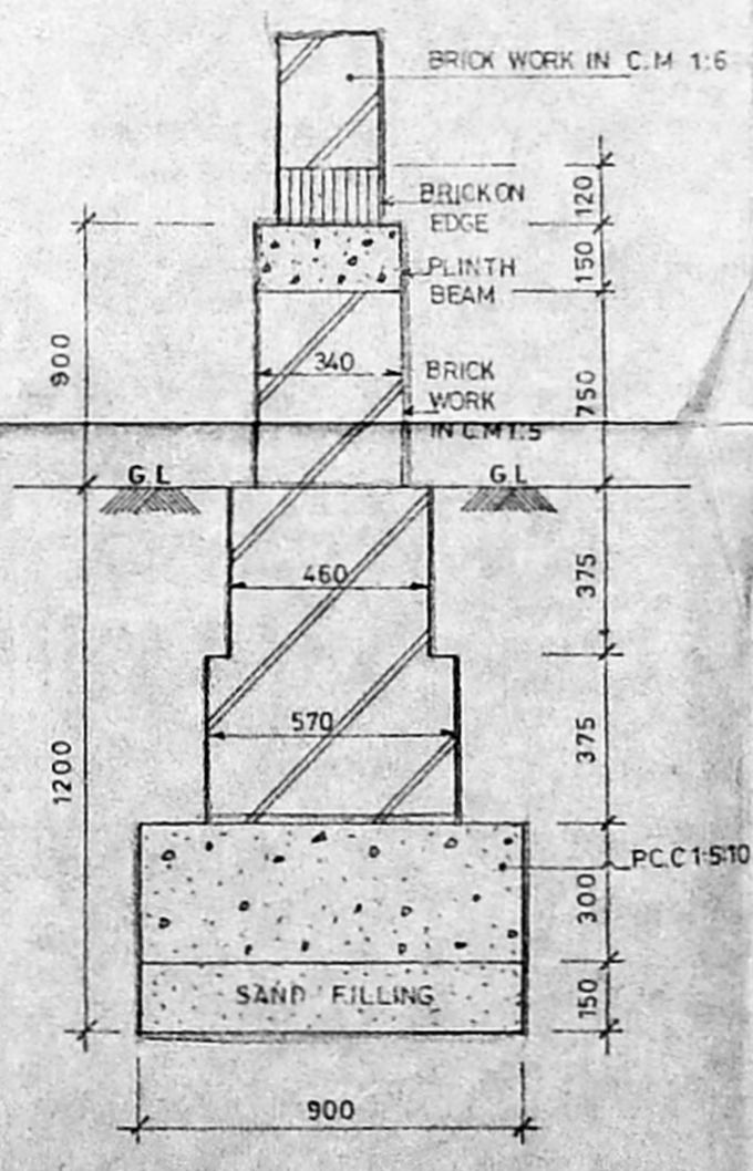
FOUNDATION DETAIL
