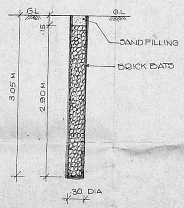
DETAIL OF RAIN WATER PERCOLATION PIT
